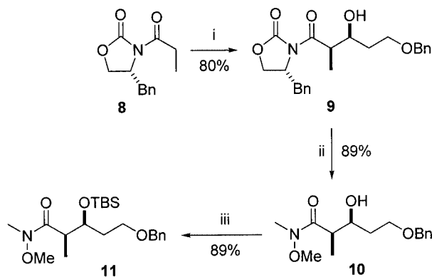
Scheme 3. Reagents: i) 8 , Bu_2BOTf , Et_3N , CH_2Cl_2 , T < 2 °C; then BnOCH_2CH_2CHO , -77 °C. ii) MeOMeNH\cdot HCl , AlMe_3 , THF , 0 °C. iii) TBSOTf, 2,6-lutidine, CH_2Cl_2 , 0 °C.
