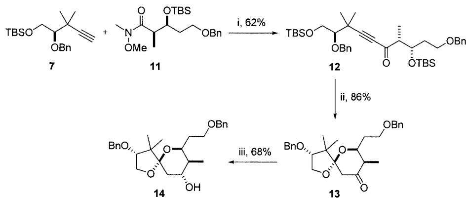
Scheme 4. Reagents: i) BuLi, 7 , then 11 , THF -78^{\circ}\text{C} . ii) CSA, MeOH, then p TsOH, PhH, room temp. iii) L-Selectride, THF, -78^{\circ}\text{C} .
