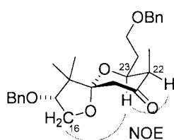
Figure 3. Double-pulsed field-gradient spin-echo (DPGFSE) NOE experiment.
