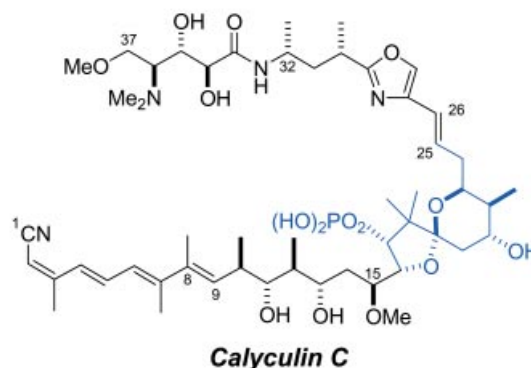
Figure 1. Spiroketal fragment of calyculin C.
