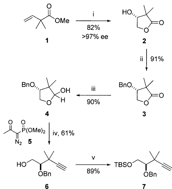
Scheme 2. Reagents: i) DHQ-PYR, K_3Fe(CN)_6 , K_2CO_3 , H_2O/tBuOH (1:1), OsO_4 , 0 °C. ii) CH_2Cl_2/cyclohexane (1:3), benzyl 2,2,2-trichloroacetimidate, CF_3SO_3H , 35 °C. iii) DIBAL-H, PhMe , -78 °C. iv) 5 , K_2CO_3 , MeOH , 36 °C. v) TBSOTf, 2,6-lutidine, CH_2Cl_2 , 0 °C.
