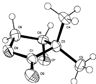
Figure 2. Crystal structure of lactone 2 .
