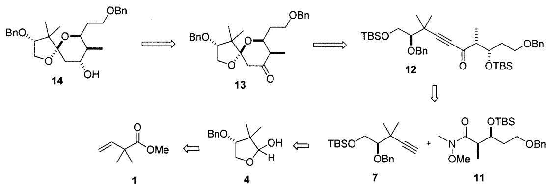
Scheme 1. Retrosynthetic analysis for the spiroketal fragment 14 .
