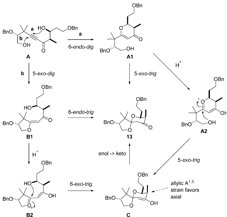
Scheme 5. Possible reaction pathways.
