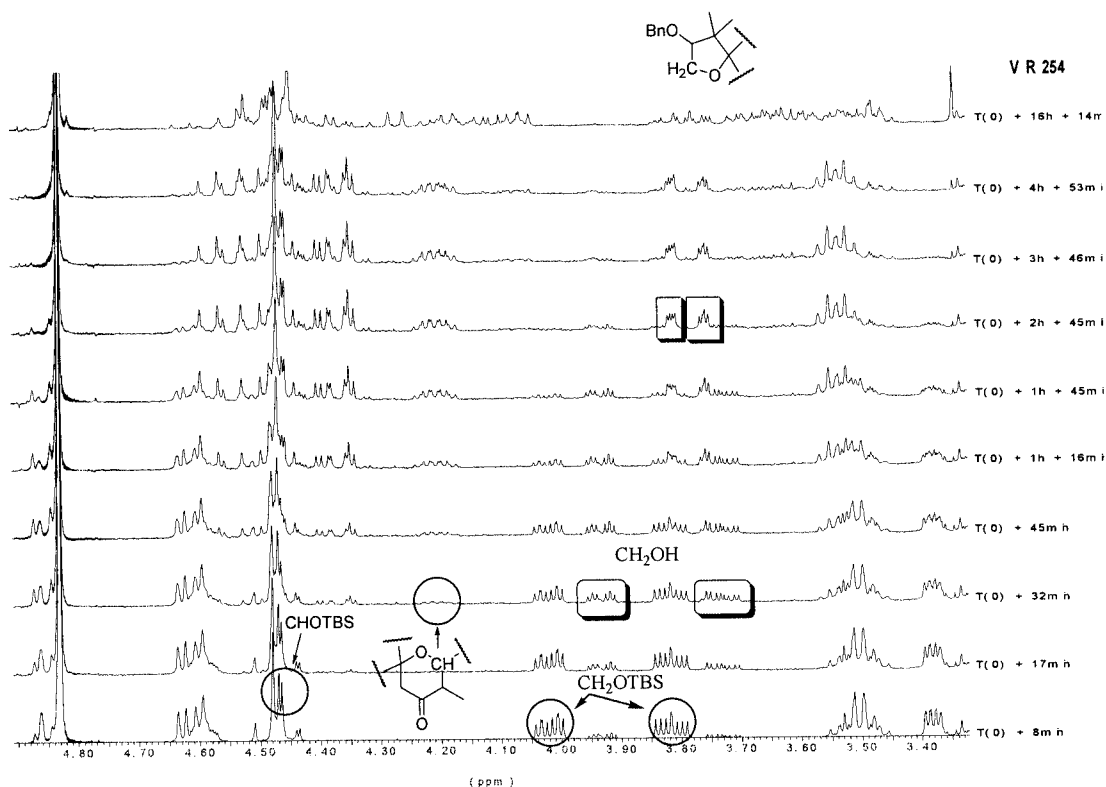
Figure 4. Reaction T(0) + 8 min to T(0) + 16 h 14 min.
